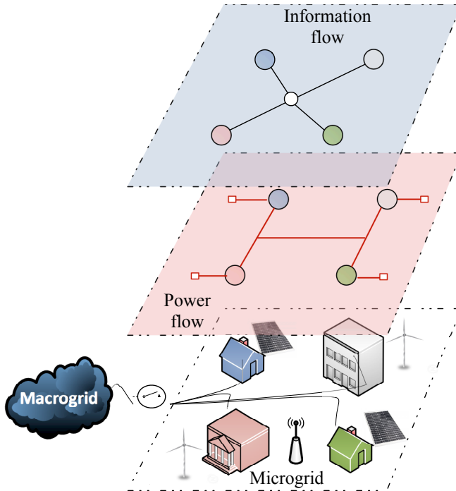
Fig. 5. Example of microgrid [11].
