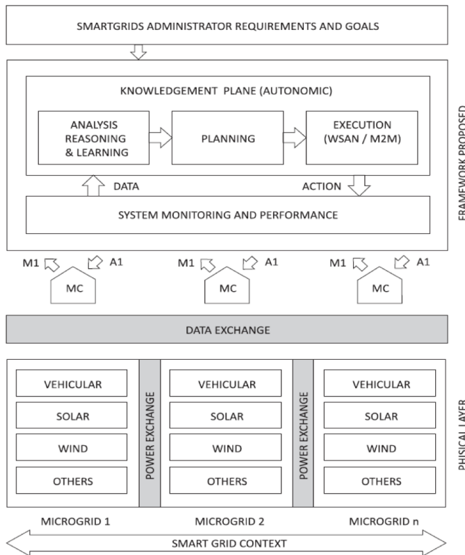
Fig. 10. Proposed Framework to Support Smart Grid Solutions.
