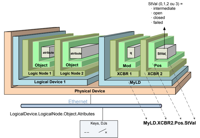
Fig. 9. Example of a name reference objects of IEC 61850 and its hierarchical structure.
