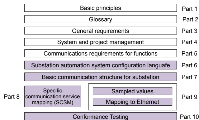
Fig. 8. Composition of IEC 61850 standard [36].
